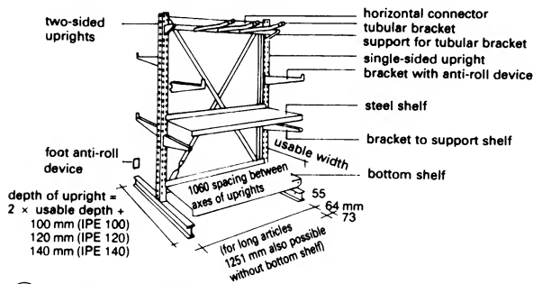
3 Bracket rack system
